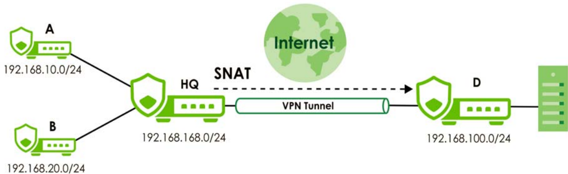
Figure 79 Policy Based VPN - SNAT Example Scenario
