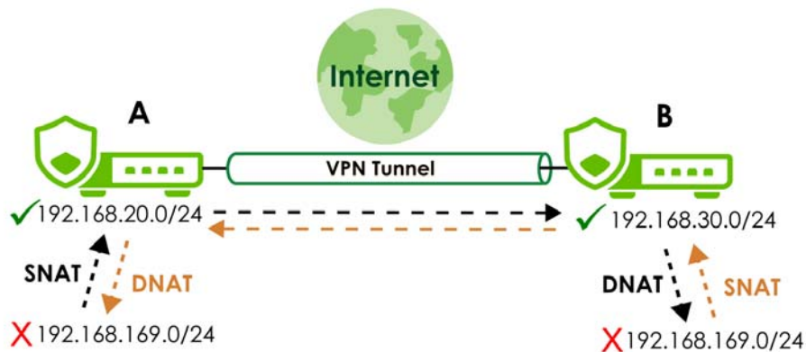
Figure 80 Policy Based VPN - 1:1 NAT Example Scenario
