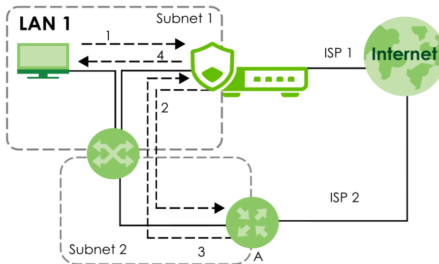
Figure 75 Using Virtual Interfaces to Avoid Asymmetrical Routes
