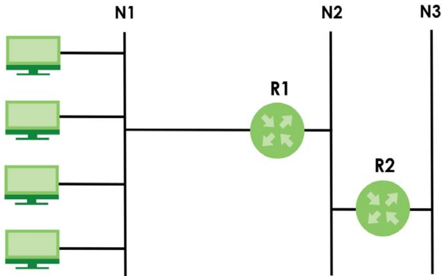
Figure 72 Example of Static Routing Topology
